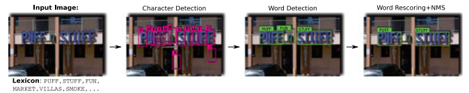
Fig. 4. Illustration of a word spotting approach [148]. Characters are recognized with HOG features and Random Ferns classifiers, and words are modeled with a pictorial structure model (Courtesy of K. Wang).
