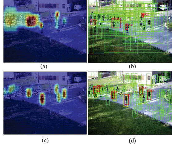
Figure 2. Object discovery from noisy proposals. (a) The score map in the first learning iteration and (b) candidate objects (red boxes) discovered. (c) The score map and in the fifth learning iteration. (d) Candidate objects (red boxes) and hard negatives (yellow boxes). (Best viewed in color.)
