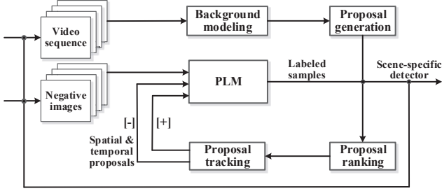
Figure 3. Block diagram of the proposed self-learning approach
