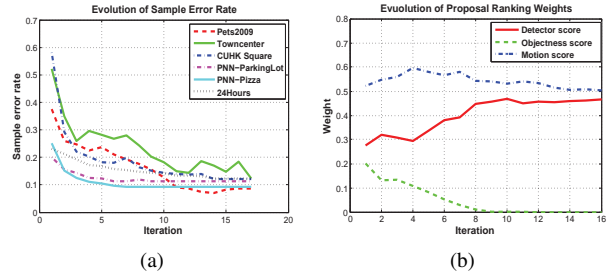
Figure 5. Validation of learning stability. (a) Monotonical decrease of sample error rates. (b) Evolution of proposal ranking weights.
