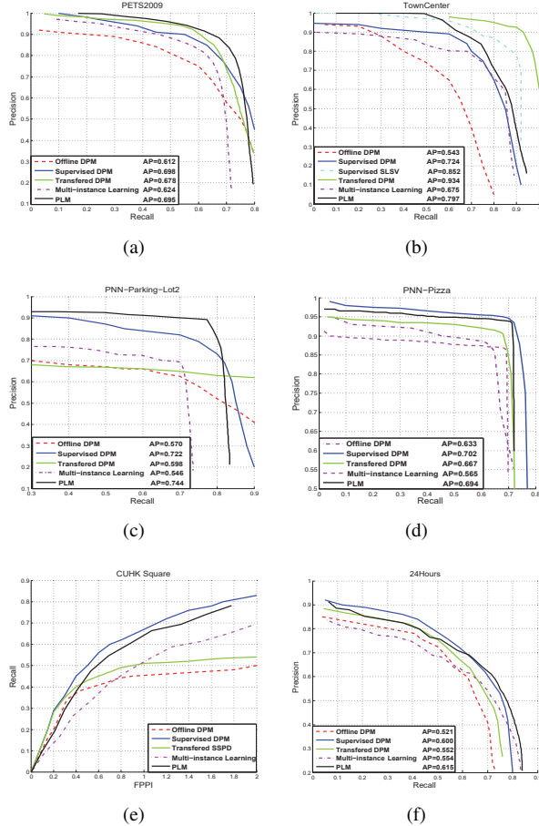
Figure 6. Performance of our approach and comparisons with weakly supervised, supervised, and transfer learning approaches. On five datasets the Precision-Recall metric is adopted to evaluate the approach and compare it with other approaches. On the CUHK dataset the FPPI-Recall metric is adopted, consistent with the state-of-the-art scene-specific detection approach [37].
